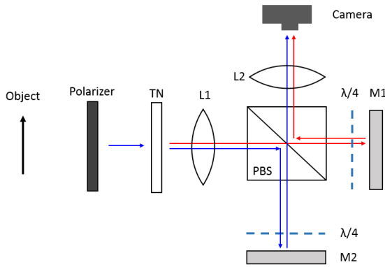
Fig. 1. Experimental setup to realize path length difference for two different polarizations using a PBS. The two paths for s- and p- polarizations are denoted as red and blue arrows. The path difference is introduced by placing mirrors M1 and M2 at different distances from PBS.
