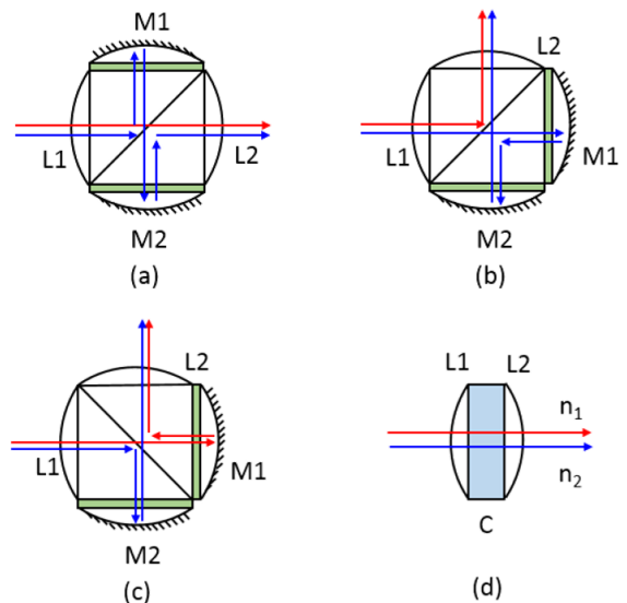
Fig. 4. Four possible device configurations with more versatility. In (a)–(c), green blocks represent the \lambda/4 films. In (d), the blue block, C, denotes a uniaxial/biaxial plate.
