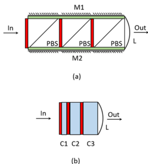
Fig. 5. Two examples of the stacked device that has 2^3 possible focuses. Red bars indicate the location of TN cells. Green blocks in (a) represent the \lambda/4 films and the blue blocks in (b) stand for the uniaxial/biaxial plates.
