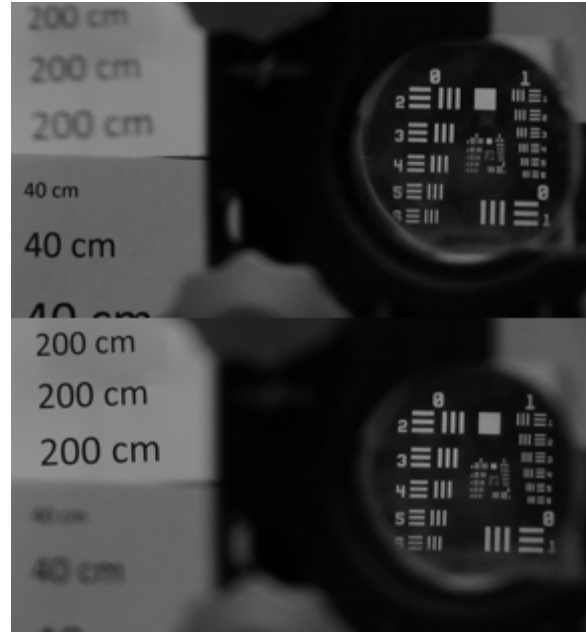
Fig. 3. Experimental results for the setup shown in Fig. 1 without L1 and with new configuration (see text). When switching on/off the TN cell, we can switch the image between 40 cm and 200 cm while retaining its angular size.
