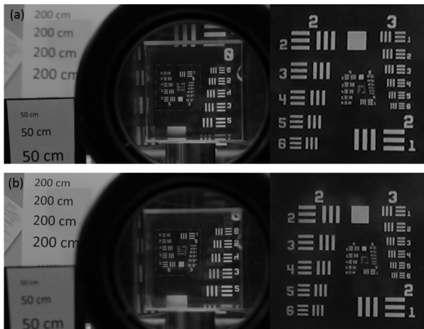
Fig. 2. When looking into the PBS, the switching between two paths results in different images. Photo (a) shows the image corresponding to the red line in Fig. 2; the image was located at 50 cm away from the camera. Photo (b) shows the image corresponding to the blue line in Fig. 2; the image was located at 200 cm away. The other images beside the main images are results of surface reflection from other components. Photos on the right side are the enlarged and inverted pictures of the red dashed blocks.
