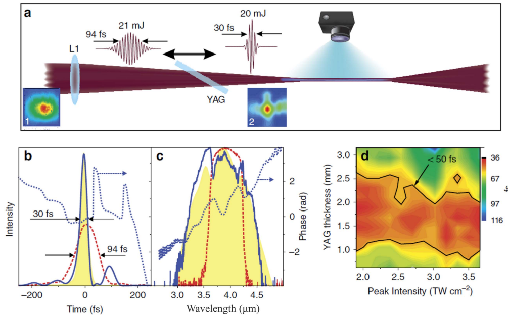
Figure 17. Setup for self-compression and characterization of mid-infrared pulses. (a) Sketch of the experimental setup: three-fold self-compression of 94 fs, 21 mJ pulses, centered at 3.9 \mu\text{m} , is achieved in a 2 mm thick YAG plate placed at a certain distance from the focusing lens L1; (b), (c) retrieved from SHG FROG measurements temporal (b) and spectral (c) pulse profiles of the output of 3.9 \mu\text{m} OPCPA system (dashed red line) and self-compressed in YAG pulses (blue solid line); the yellow area represents calculated temporal profile and spectrum of the self-compressed pulse (normalized intensity). Dotted blue lines show retrieved temporal and spectral phases; (d) 3D-map representing the dependence of the output pulse duration on the thickness of the material and on the input peak intensity. Reproduced from [83]. CC BY 3.0.
