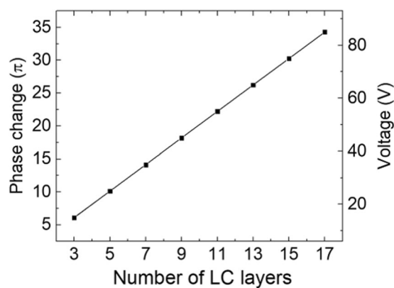
Figure 2. The simulated correlation between number of LC layers ( N ), driving voltage and phase change at 633\ \text{nm} with each layer being 2.2\ \mu\text{m} . At N=6 , the phase change reaches 12.1\ \pi at 30\ V_{\text{rms}} for \lambda = 633\ \text{nm} , which corresponds to \delta = 2.0\ \pi at \lambda = 3\ \mu\text{m} .
