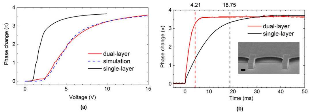
Figure 3. A dual-layer ( N=2 ) sample compared to a conventional single-layer sample with the same effective cell thickness of 3.4\ \mu\text{m} . (a) The measured and simulated voltage dependent phase change of the single-layer and double-layer samples at \lambda=633\ \text{nm} . (b) The relaxation time of phase change from 0–90% for dual and single layer samples are 4.21 ms and 18.75 ms, respectively. Inset: the SEM image of a dual-layer sample, scale bar: 2\ \mu\text{m} .
