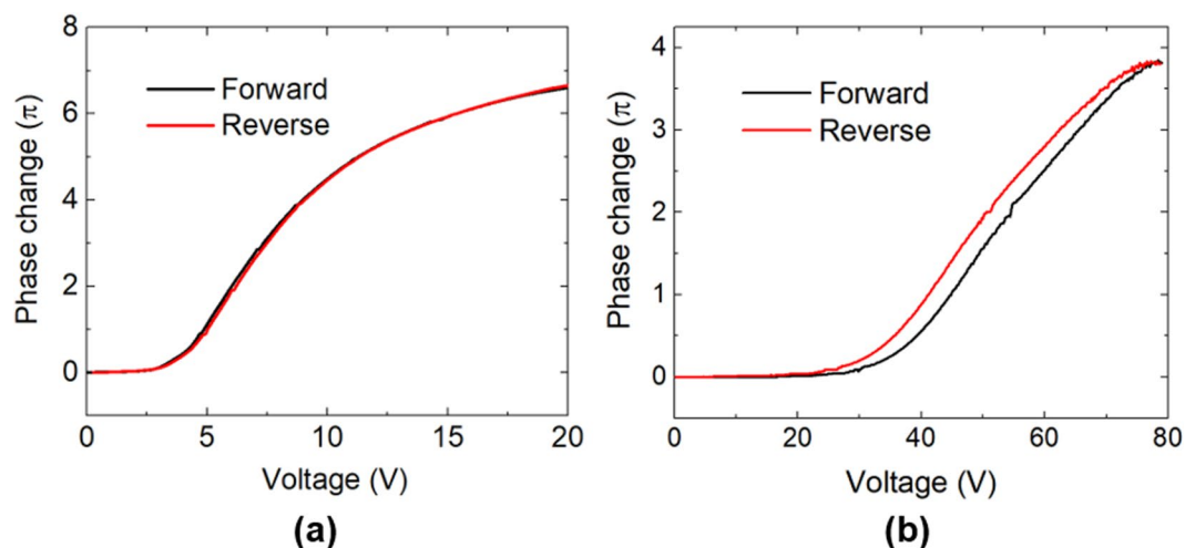
Figure 6. Hysteresis of (a) MLC and (b) PNLC. The discrepancy between forward and reverse processes shows visible hysteresis for a typical PNLC.
