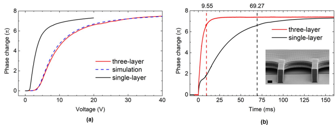
Figure 4. A three-layer ( N = 3 ) sample compared to a conventional single-layer sample with the same effective cell thickness of 6.6 \mu\text{m} . (a) The voltage versus phase change shows a phase change of 7.2\pi at 30 V_{\text{rms}} . \lambda = 633 \text{ nm} . (b) The relaxation time of phase change from 0–90% for the three- and single-layer samples are 9.55 ms and 69.27 ms, respectively. Inset: the SEM image of a three-layer sample, scale bar: 2 \mu\text{m} .
