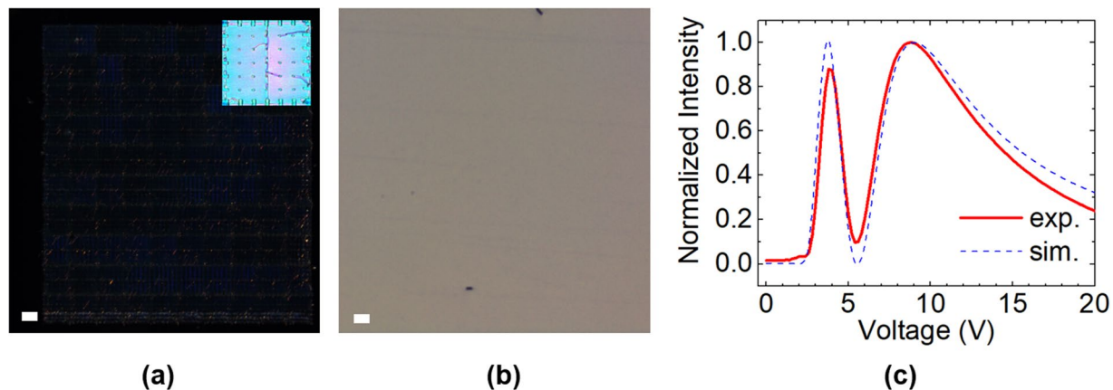
Figure 5. The dark-field micrographs of (a) a three-layer sample and (b) a PNLC sample at 40 V_{\text{rms}} , showing a reduced scattering for MLC. (c) The voltage-transmittance curve ( \lambda = 633 \text{ nm} ) of a two-layer MLC sample between crossed polarizers, showing the scattering-induced discrepancy between the experimental and simulation results. Scale bar: 50 \mu\text{m} . Inset: the bright-field micrograph of the three-layer sample.
