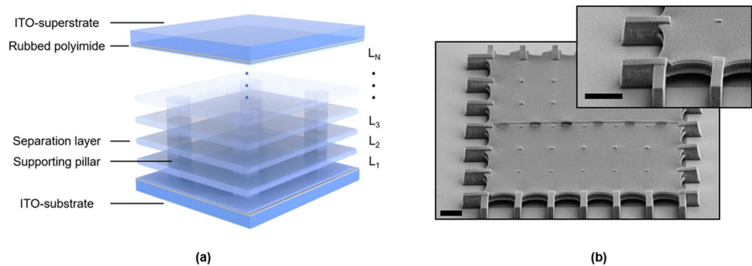
Figure 1. (a) Illustration of the multi-layer structure with N being the number of liquid crystal layers. (b) The SEM image of a three-layer LC cell. Scale bar: 10\ \mu\text{m} .
