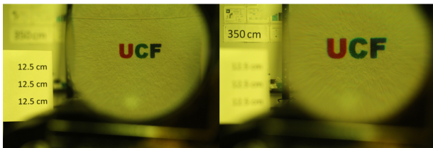
Figure 7: When looking into the PBL and the offset lens, the switching of voltage-on and voltage-off states upon PBL results in different image distances as shown above. The left photo shows the image when the PBL is in voltage-off state (image located at 12.5 cm), while the right photo shows the image in voltage-on state (image located at 350 cm).
