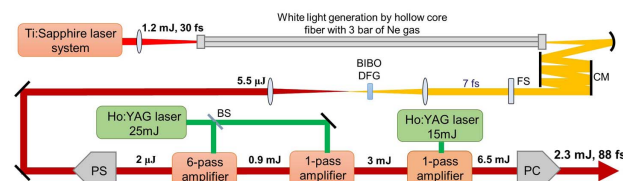
Fig. 1. Schematic layout of the Cr 2+ :ZnSe CPA laser. CM, chirped mirrors; FS, fused silica compensation plate; DFG, difference frequency generation; PS, pulse stretcher; PC, pulse compressor.
