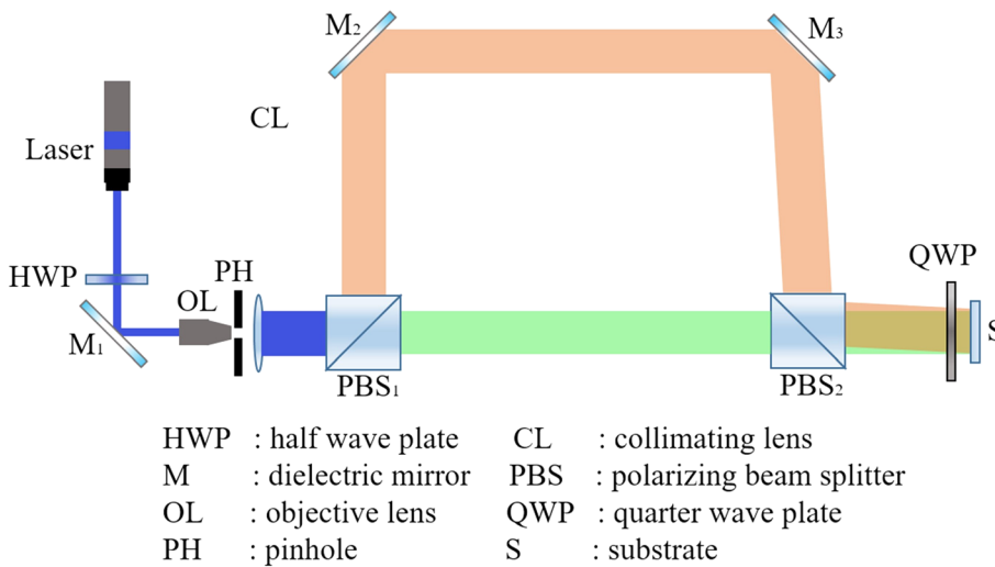
FIGURE 8 Experiment setup for polarization holographic recording of the PBD. PBD, Pancharatnam-Berry deflector
