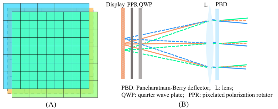
FIGURE 3 (A) The original panel (orange) is separated into two virtual panels (blue and green); the new half pixel pitch grid (cyan) is formed by superimposing two virtual panels. (B) Schematic illustration of the resolution-enhanced near-eye display system based on polarization multiplexing
