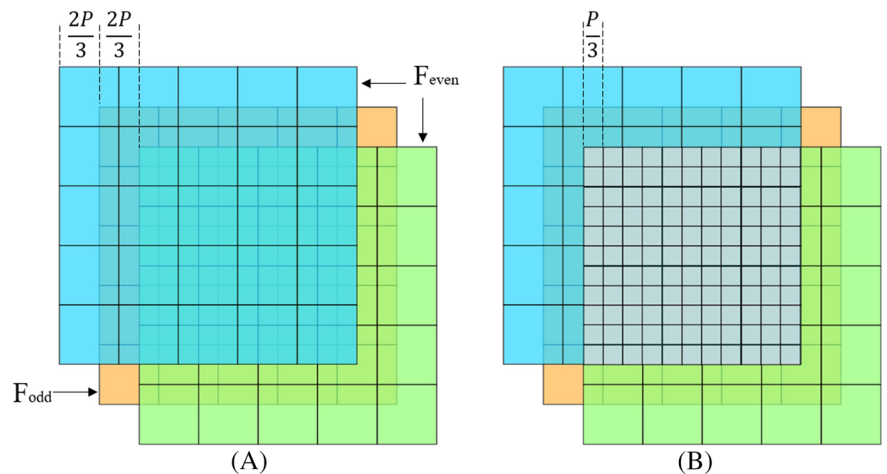
FIGURE 11 Operation principle of the shifted superimposition method to triple the resolution density. (A) The original panel (orange) presents at odd frames ( F_{odd} ), and the shifted panels (green and blue) present at even frames ( F_{even} ). (B) A new pixel grid (gray) with one third pixel pitch ( P/3 ) is formed by superimposing three panels
