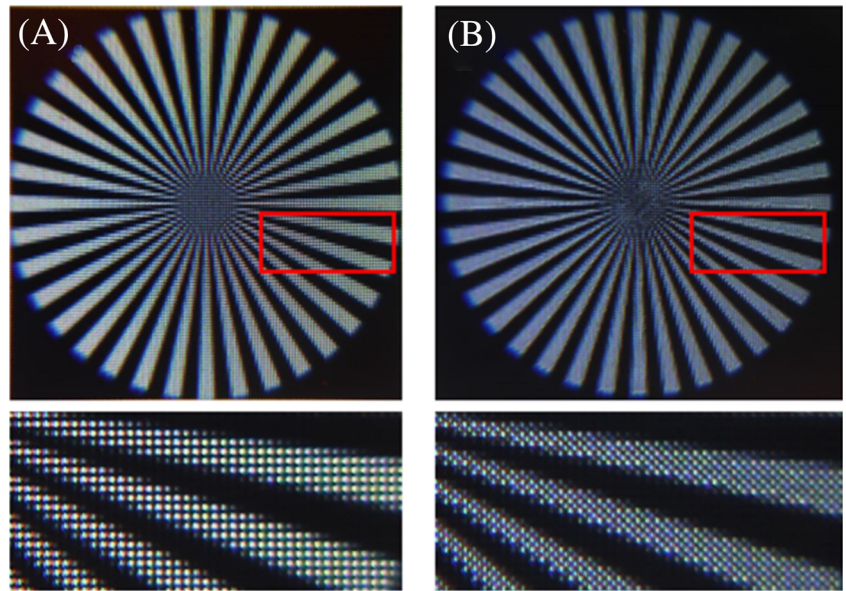
FIGURE 6 Captured images of (A) original and (B) enhanced resolution of a “Siemens star” resolution target
