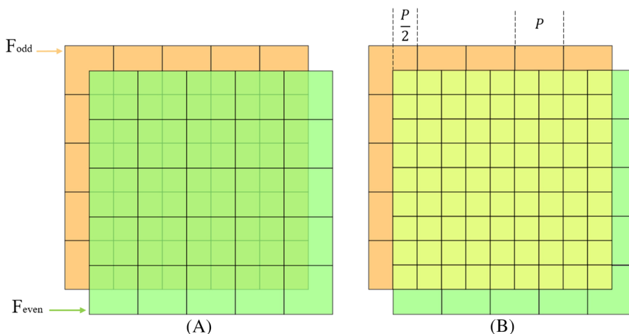
FIGURE 2 Operation principle of the shifted superimposition method to improve the resolution density. (A) The original panel (orange) presents at odd frames ( F_{\text{odd}} ), and the shifted panel (green) presents at even frames ( F_{\text{even}} ). (B) A new pixel grid (yellow) with half a pixel pitch ( P/2 ) is formed by superimposing two panels
