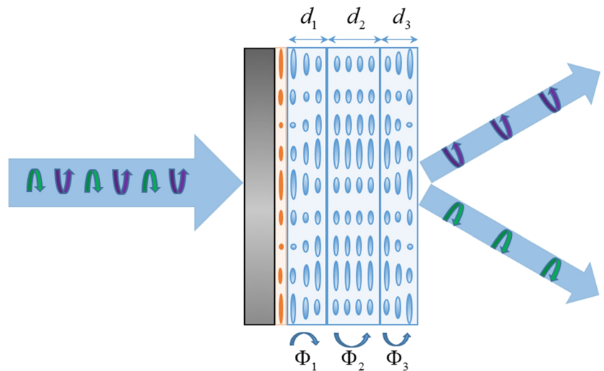
FIGURE 7 Structure of three-layer multi-twist PB phase grating. PB, Pancharatnam-Berry
