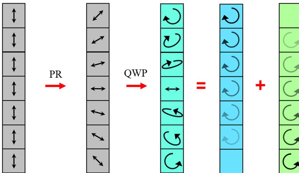
FIGURE 5 Illustration of polarization states through the PML. PML, polarization modulation layer; PR, polarization rotator; QWP, quarter-wave plate
