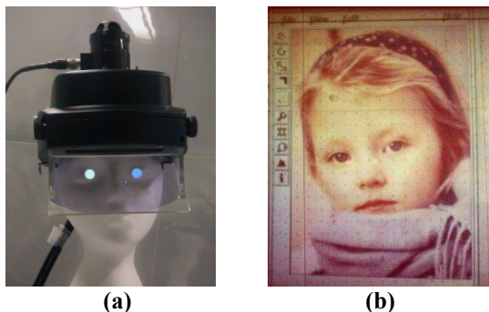
Fig. 5 Demonstrating a compact HMPD prototype: (a) Front view of the prototype; (b) Image viewed through the exit pupil of the HMPD
