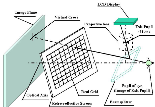
Fig. 8 Illustration of the HMPD calibration method
