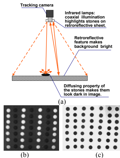
Fig. 7 A vision-based object tracker to detect physical stone locations: (a) Setup illustration: coaxial illumination highlights diffusing stones from retro-reflective background; (b) Image of black and white stones on retro-reflective background in normal lighting condition; (c) Image of black and white stones on retro-reflective background in dimmed room light with co-axial illuminators.
