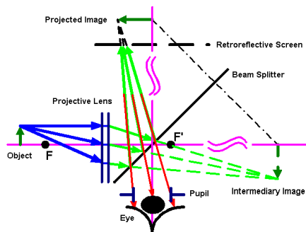
Fig.2 Imaging concept of HMPD
