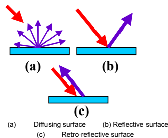
Fig. 3 Behavior of different reflective surfaces.
