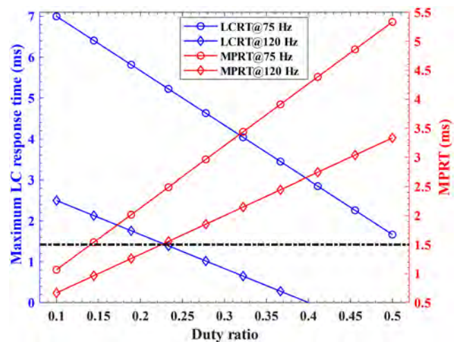
FIGURE 4 Calculated maximum allowable liquid crystal (LC) response time and the corresponding motion picture response time (MPRT) as a function of duty ratio. The gate scan time is assumed to be 5 ms. The black dashed lines represent a cathode ray tube (CRT)-like MPRT = 1.5 ms
