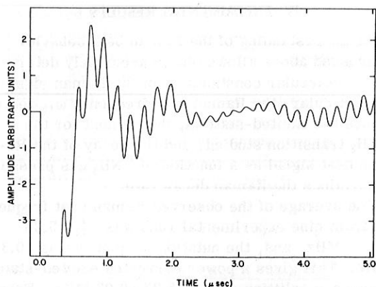
FIG. 4. Numerical solution of the three-level problem using parameters which approximate those of the upper trace in Fig. 3.
