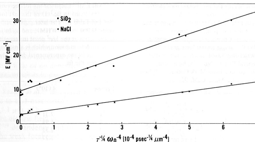
FIG. 2. rms breakdown electric field data for Harshaw single-crystal laser-grade NaCl and for General Electric high-purity water-free fused quartz is plotted as a function of t_p^{-1/4}\omega_0^{-4} where t_p is the laser pulse width (FWHM) in psec and \omega_0 is the focal-spot radius at the 1/e^2 point in intensity in \mu\text{m} . The solid lines are least-squares fits of the data to straight lines.
