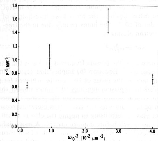
FIG. 4. Representative plot of the inverse of the power, P_B , needed to induce breakdown vs \omega_0^{-2} , where \omega_0 is the 1/e^2 radius in intensity at the laser focus calculated using linear Gaussian optics. Here data for \text{SiO}_2 using 44-psec (FWHM) pulses are presented.
