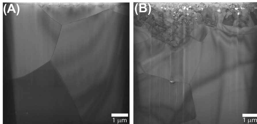
Fig. 1. (A) Cross-section of control CLS sample. (B) Cross-section of thermally annealed CLS sample showing recrystallized grains and sub-micron scale pores near the surface.
