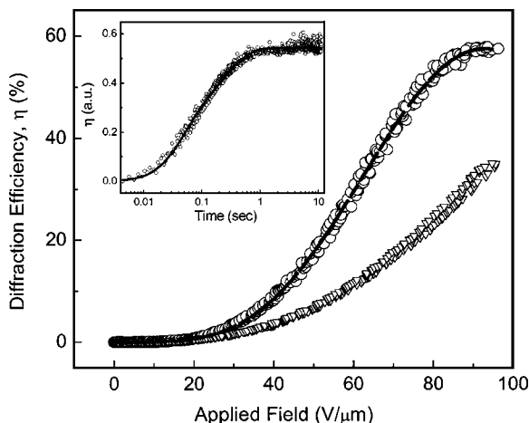
FIG. 2. Steady-state diffraction efficiency vs external electric field for C1 ( \nabla ) and C2 ( \circ ); the solid line is a theoretical fit (Ref. 14) for a trap density of 2.3 \times 10^{16} \text{ cm}^{-3} . Transient growth of diffraction efficiency as the second beam writing turned on for C2 is shown in the inset. The solid line in the inset is a biexponential growth fit ( \tau_1=33 ms, \tau_2=320 ms, weight factor m=0.5 ).
