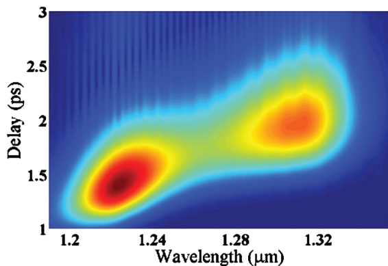
FIG. 3. (Color) WT of spectral interferogram. The maximum at each wavelength value corresponds to the group delay.
