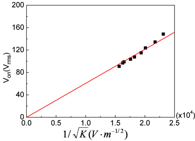
FIGURE 3 — Linear fit of V_{\text{on}} vs. K^{-1/2} according to Eq. (10) with A = 6.07 \mu\text{m}^{1/2} .
