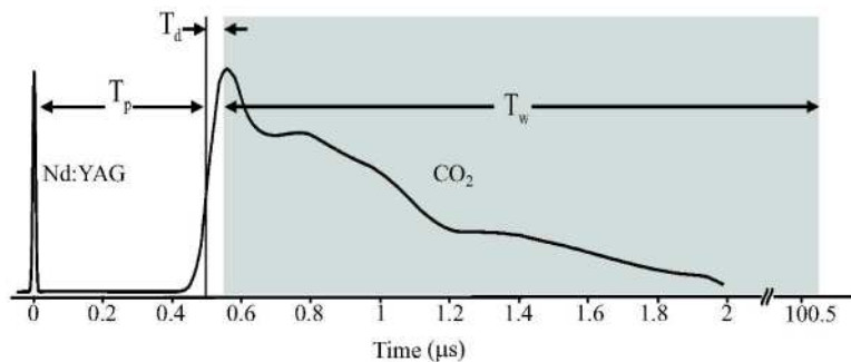
Fig. 2. The CO 2 pulse was delayed with respect to the Nd:YAG pulse by T_p and the detector gate was delayed with respect to the CO 2 pulse by T_d . The duration of the detector gate ( T_w ) was 100 μs for all cases studied
