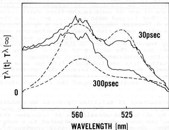
Fig. 9. A comparison of the experimental and calculated transient transmission difference spectra of a 9.2 \times 10^{-4} M solution of aqueous rhodamine B for time delays of 30 and 300 psec.
