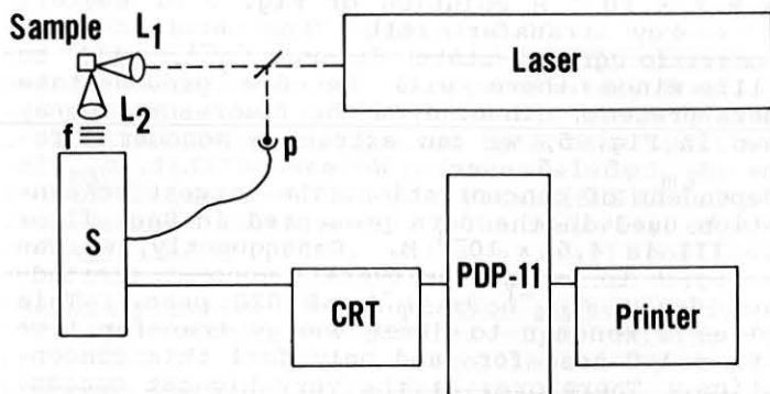
Fig. 4. Experimental arrangement for subnanosecond time-resolved fluorescence measurements.
