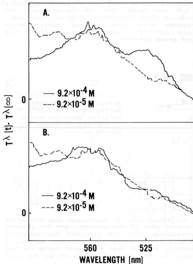
Fig. 10. A comparison of the transient transmission difference spectra (a) of dilute and concentrated solutions of rhodamine B both taken 30 psec after excitation and (b) of the dilute solution 30 psec after excitation and the concentrated solution 300 psec after excitation.
