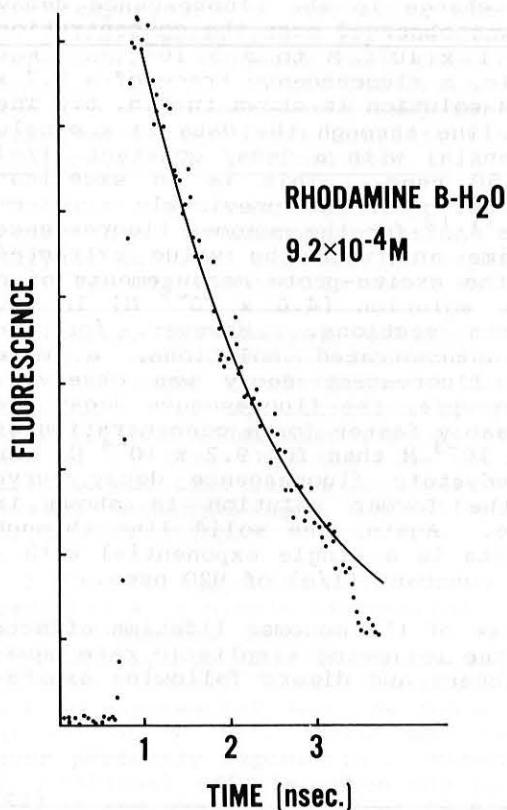
Fig. 5. Temporally-resolved fluorescence of a 9.2 \times 10^{-4} M solution of aqueous rhodamine B.
