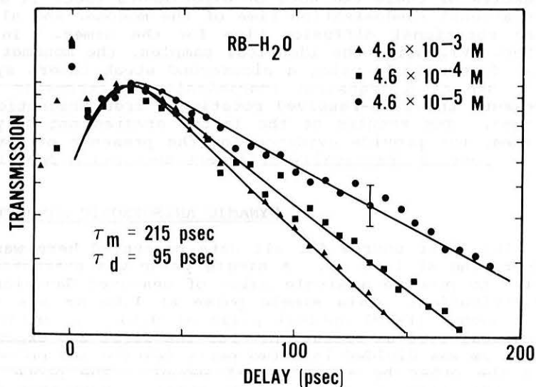
Fig. 2. The probe pulse transmission, in arbitrary units, as a function of time delay between excite and probe pulses for the geometry in Fig. 1a and for three concentrations of rhodamine B in H 2 O: 4.6 \times 10^{-3} M, 4.6 \times 10^{-4} M, and 4.6 \times 10^{-5} M. The solid lines are numerical fits to the data, as discussed in the text. Two intermediate concentrations are not shown for clarity.
