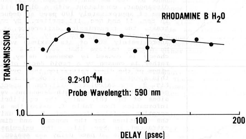
Fig. 8. Transient transmission (in arbitrary units) of a 9.2 \times 10^{-4} M solution when the probe wavelength is chosen to be 590 nm.
