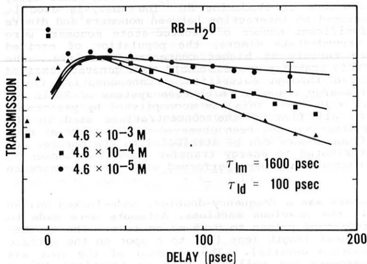
Fig. 3. The probe pulse transmission, in arbitrary units, as a function of time delay between excite and probe pulses for the geometry of Fig. 1b and for three concentrations of rhodamine B in H_2O : 4.6 \times 10^{-3} M , 4.6 \times 10^{-4} M , and 4.6 \times 10^{-5} M . The solid lines are numerical fits to the data, as discussed in the text. Two intermediate concentrations are not shown for clarity.
