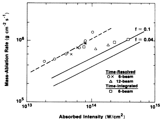
FIG. 4. Mass-ablation rate versus absorbed intensity at \lambda=0.351 \mu\text{m} . Compilation from this study (---), time-integrated measurements from Ref. 6, and LILAC simulations at f=0.1 and 0.04 for the rising edge of the pulse.
