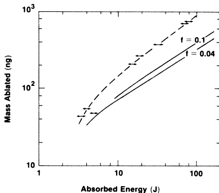
FIG. 3. Ablated mass vs absorbed energy during a single laser pulse for six-beam irradiation of multilayer targets. Solid lines are LILAC simulations for the mass outside the 500-eV isotherm. For the experimental data the total mass outside the glass substrate is assumed to have been ablated. Data points at \sim 4 J absorbed energy are for the ablation of the outer Au layer only.
