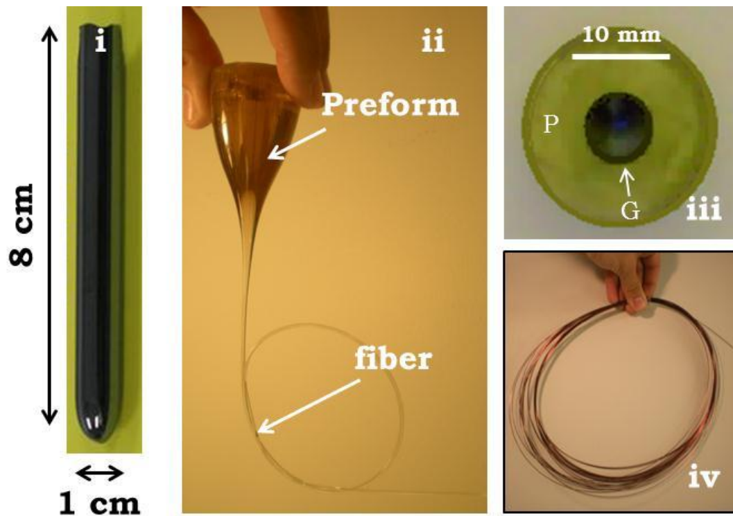
Figure 1 Preform preparation and fiber drawing to produce in-fiber micro-wires. Optical images of (i) a glass rod used as the core; (ii) a preform after TFD; (iii) the preform cross section; and (iv) a 10-m-long drawn fiber containing ~ 27,000 200-nm-diameter nanowires.
