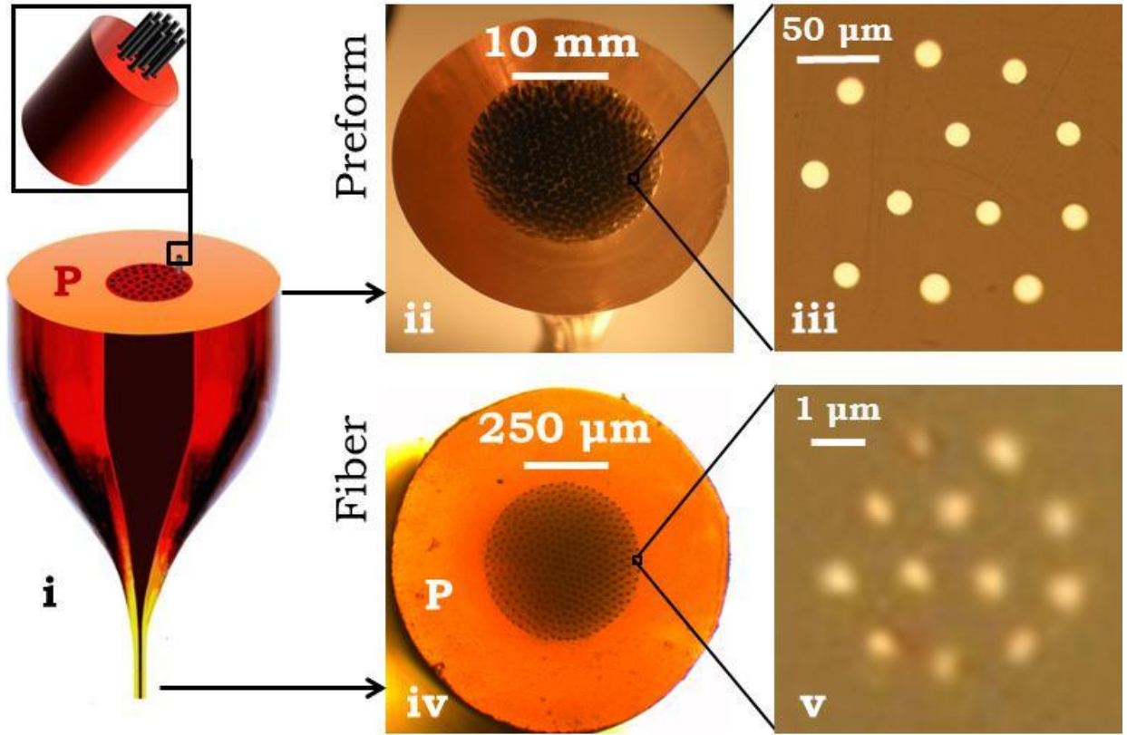
Figure 2. Stack-and-draw of a high-density well-ordered array of nanowires. (i) Schematic of the drawn preform. (ii) Photograph of the stacked preform cross section and (iii) a reflection optical micrograph of an individual fiber in the stack containing 12 \text{As}_2\text{Se}_3 cores (from a previous stack-and-draw step). (iv) Transmission optical micrograph of the drawn fiber cross section. (v) Reflection optical micrograph showing the 12 500-nm-diameter \text{As}_2\text{Se}_3 cores maintaining the same configuration in iii.
