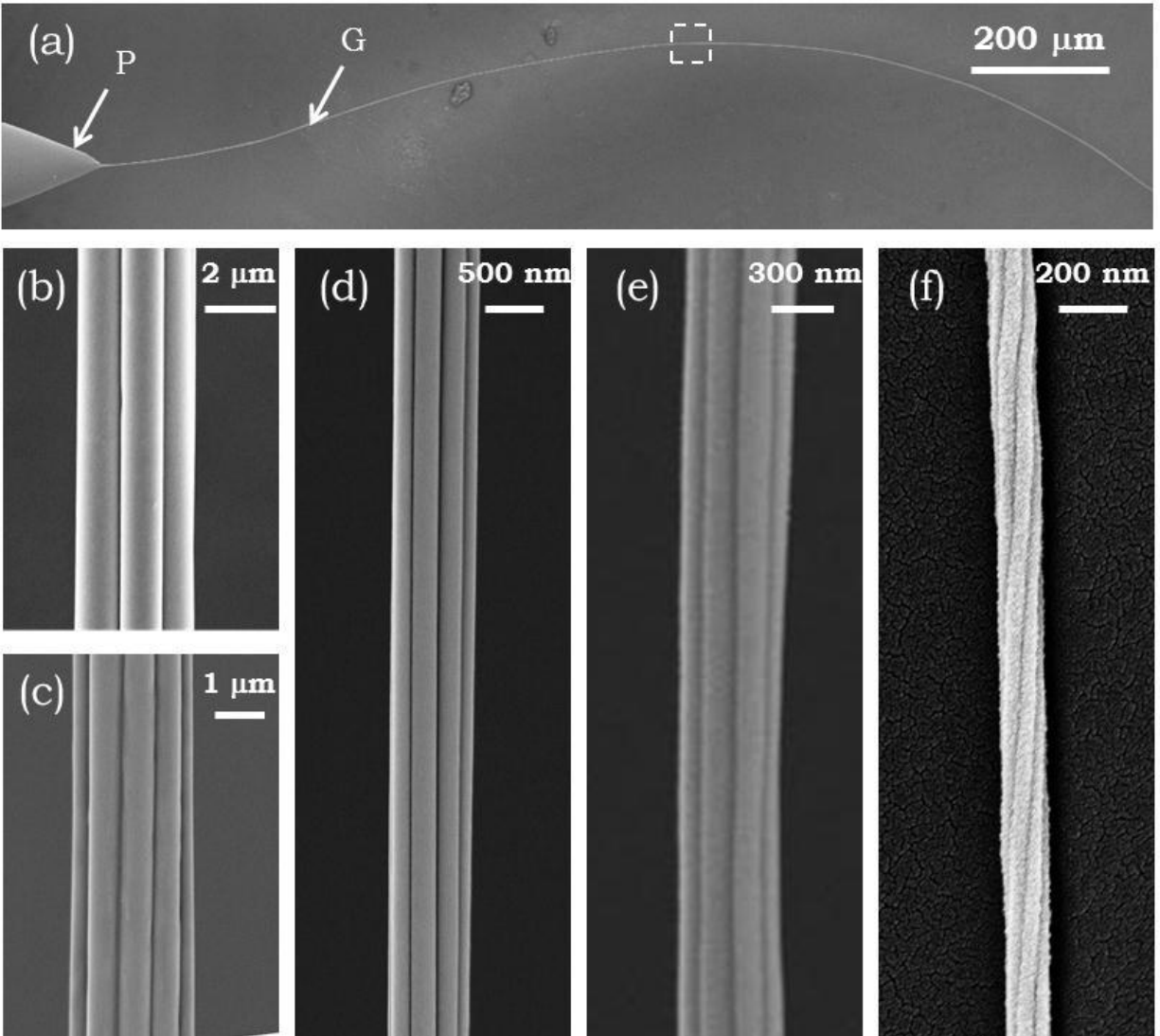
Figure 3. In-fiber nanowire arrays produced by TFD. (a) SEM micrograph demonstrating the continuity and robustness of an exposed nanowire array (500-nm-diameter cores) emerging from the fiber tip after dissolving the polymer cladding. (b)-(f) SEM micrographs of nanowire arrays with individual diameters (b) 1 μm, (c) 650 nm, (d) 200 nm, (e) 100 nm, and (f) 50 nm.
