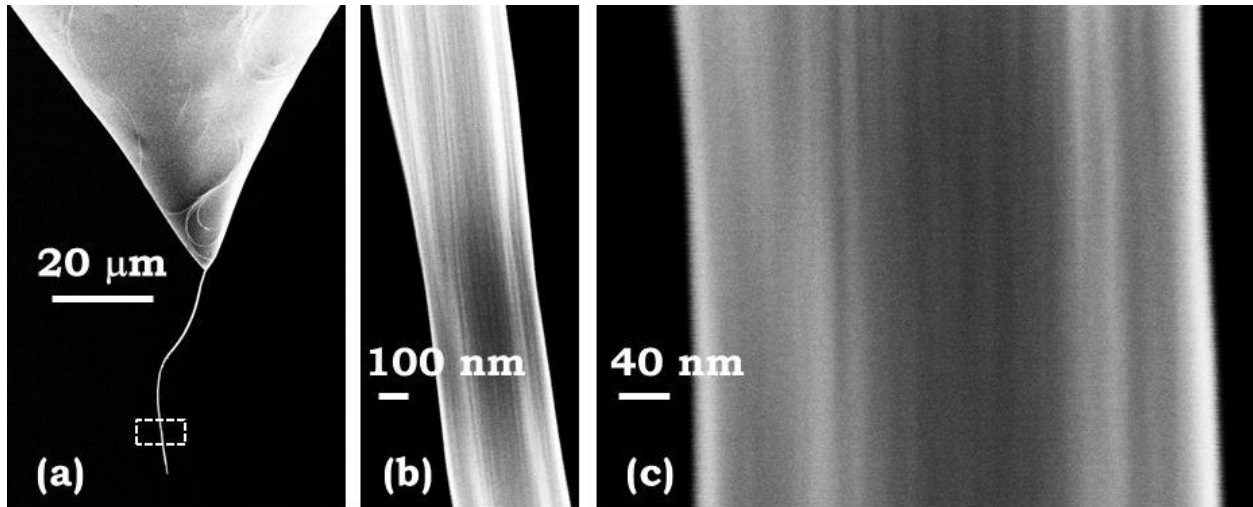
Figure 4. 2.5-nm-diameter high-density nanowire arrays produced by tapering a fiber containing 20-nm-diameter nanowires. (a) SEM micrograph of an intact exposed bundle of 2.5-nm-diameter nanowires emerging from the tapered fiber tip. (b) SEM micrograph of the dashed white box in (a), and (c) a zoomed-in SEM micrograph of (b), both showing continuous bundles of nanowires. The visible strands are most likely the sets of 12 2.5-nm-diameter nanowires.
