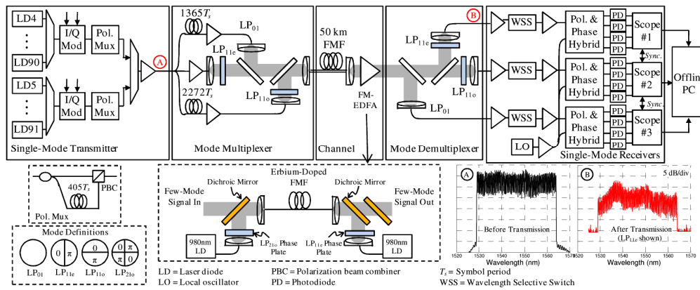
Fig. 5. Experimental setup.
