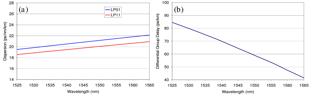
Fig. 14. Predicted (a) differential mode group delay and (b) chromatic dispersion.
