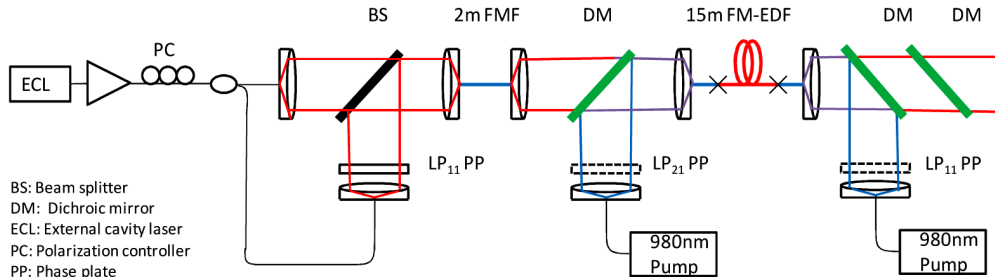
Fig. 2. Experiment setup.
