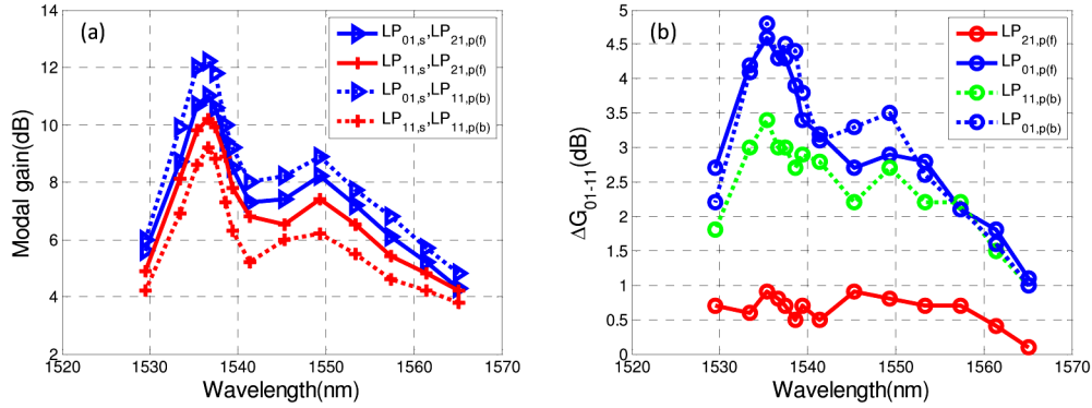
Fig. 4. (a) Modal gain vs. signal wavelength, using LP 21,p (forward) and LP 11,p (backward) and (b) MDG vs. signal wavelength using forward pumps in LP 01,p , LP 21,p and backward pumps in LP 01,p , LP 11,p .
