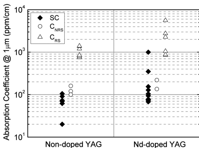
FIG. 2. Absorption coefficient of non-doped YAG (left halves) and Nd-doped YAG (right halves) ceramics and single crystals at 1064 \text{ nm} . Closed diamonds, open dots, and open triangles represent single crystals (SC), non-reactively sintered ceramics ( C_{\text{NRS}} ), and reactively sintered ceramics ( C_{\text{RS}} ), respectively.
