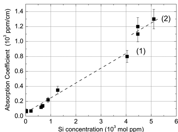
FIG. 4. Dependence of 1 \mu\text{m} absorption coefficient of different YAG samples on their Si impurity concentration for (1) Ca concentration [\text{Ca}] < 0.5 \text{ wt. ppm} and (2) [\text{Ca}] = 240 \text{ wt. ppm} . The dashed line is added for visualization purposes.
