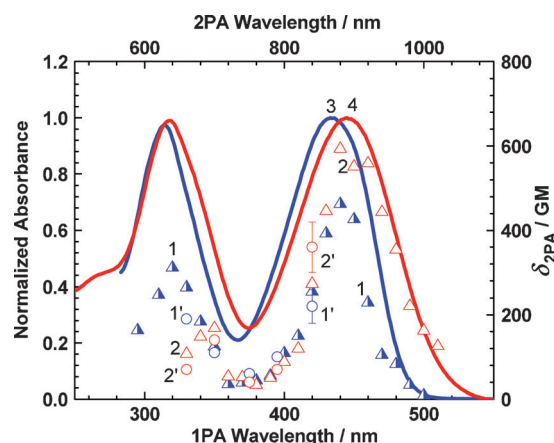
Figure 5. Degenerate 2PA spectra of 1 in TOL (1, 1') and \text{CHCl}_3 (2, 2'), obtained by 2PF (1, 2: triangles) and open-aperture Z-scan (1', 2': circles) methods. Normalized linear absorption spectra of 1 in TOL (3) and \text{CHCl}_3 (4).
