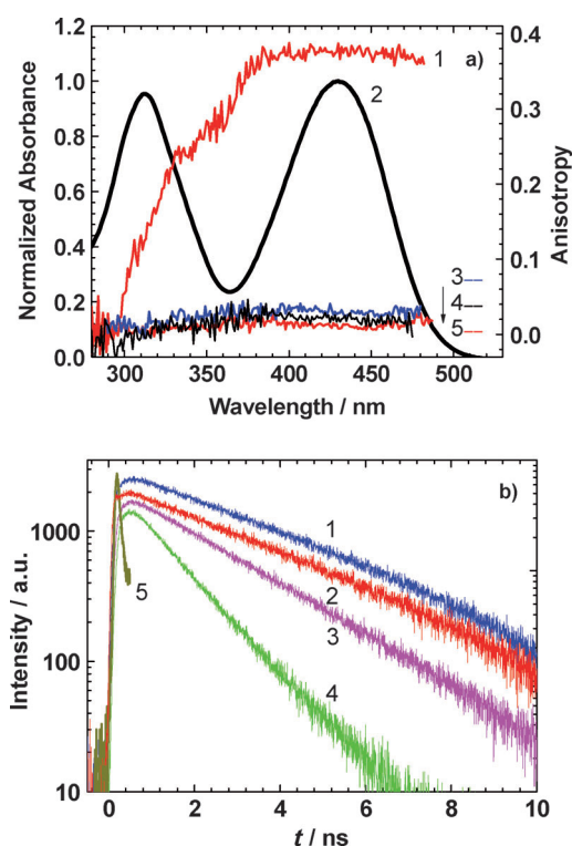
Figure 2. a) Excitation anisotropy spectra of 1 in pTHF (1), THF (5), TOL (3), HEX (4), and normalized absorbance in THF (2). b) Fluorescence lifetime decay curves for 1 in THF (1), CHCl 3 (2), TOL (3), HEX (4), and instrument response function (5).
