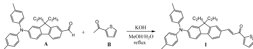
Scheme 1. Synthesis of chromophore 1 .
