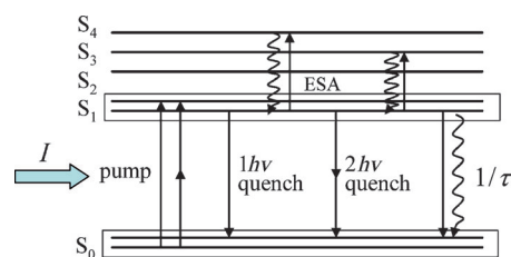
Figure 6. Main spontaneous and stimulated transitions in 1.
