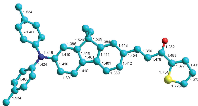
Figure 3. Optimized molecular geometry of 1 obtained with the DFT/6-31(d,p)/B3LYP method (bond lengths in Å). Ethyl groups are replaced with CH 3 for simplicity.
