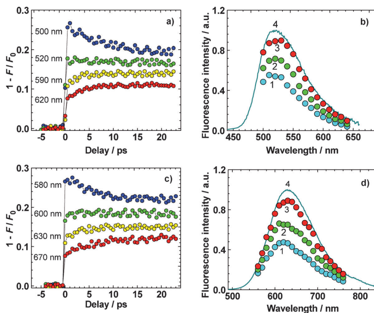
Figure 8. Transient quenching dependences 1 - I_F/I_{F0} = f(\tau_D) (a,c) of 1 in TOL (a) and \text{CHCl}_3 (c) for corresponding quenching wavelengths \lambda_q . Time-resolved one-photon STED spectra of 1 (b,d) for \tau_D = 0 \text{ ps} (1, cyan circles), 2 ps (2, green circles), and 6 ps (3, red circles) in TOL (b) and \text{CHCl}_3 (d). Normalized fluorescence spectra (b and d, curves 4) of 1 in TOL (b) and \text{CHCl}_3 (d).
