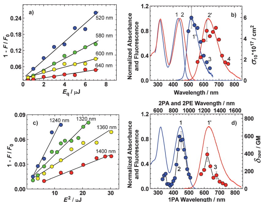
Figure 7. Fluorescence quenching dependences 1 - I_F/I_{F0} = f({}^q E_p) (a) and 1 - I_F/I_{F0} = f({}^q E_p^2) (c) of 1 in TOL (a) and \text{CHCl}_3 (c) for corresponding quenching wavelengths \lambda_q . Solid black lines are linear fittings (a,c). One-photon STED spectra of 1 (b, curves 3, 4, blue and red circles) in TOL (3, blue circles) and \text{CHCl}_3 (4, red circles). 2PA spectrum (d, curve 2) and two-photon STED spectrum (d, curve 3) of 1 in \text{CHCl}_3 . Normalized absorption spectra (b, curves 1 and 2; d, curve 1) and fluorescence spectra (b, curves 1' and 2'; d, curve 1') of 1 in TOL (b, curves 1 and 1') and \text{CHCl}_3 (b, curves 2 and 2'; d, curve 1').
