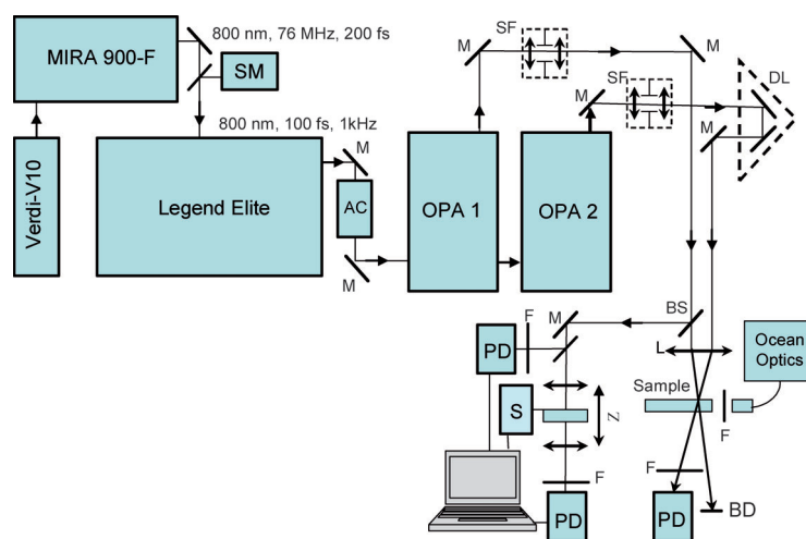
Figure 11. Simplified diagram of the experimental setup: SM: spectrometer; AC: optical autocorrelator; M: 100% reflection mirrors; BS: beam splitter; SF: space filters; DL: optical delay line with retro-reflector; PD: calibrated Si and/or InGaAs photodetectors; L: focusing lenses; F: set of neutral and/or interferometric filters; S: step motor; Sample: 1 mm flow quartz cuvette with investigated solutions; Z: Z-scan setup; BD: beam dump. Additional details are presented in the text.
