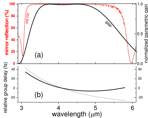
Fig. 6. (a) Reflectivity curve of the dielectric mirror (red curve) and relative parametric gain of the 0.5-mm OP-GaAs (black curve) vs. wavelength. (b) Cumulative group delay introduced by 0.5-mm GaAs plus 80- \mu\text{m} YAG plus dielectric mirror (solid curve) and group delay without YAG plate (dashed curve).
