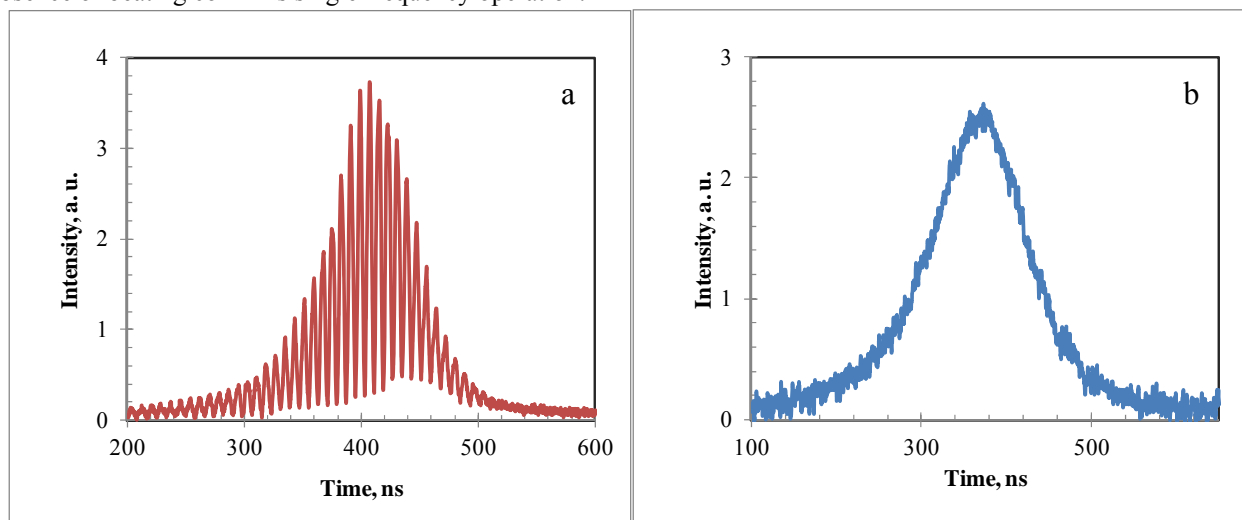
Figure 6. Temporal pulse profiles in a double (a) and single (b) frequency generation regimes
