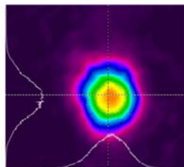
Figure 8. Far-field profile of the laser output
