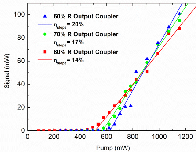
Fig. 3. Laser performance of the Cr:ZnS waveguide laser at 2332.6 nm. A maximum output power of 101 mW with a slope efficiency of 20% is demonstrated using a 60%R output coupler.
