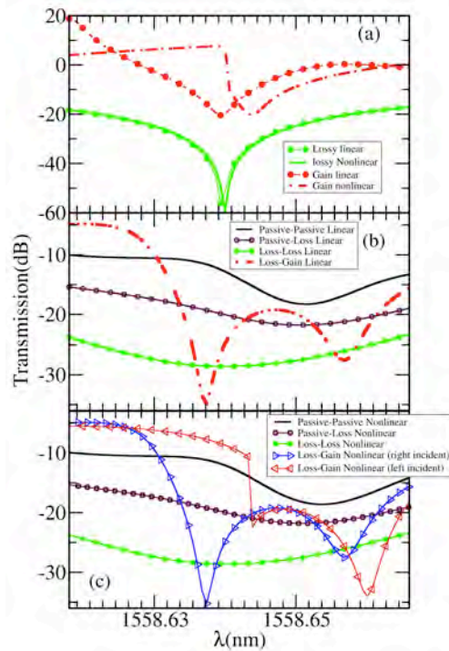
Fig. 3. (a) Transmittances T(\lambda) for a single gain or loss microdisk coupled to a waveguide. The filled green circles (green line) correspond to a lossy disk in the absence (presence) of Kerr nonlinearity. The filled red circles (dotted-dashed line) correspond to a gain disk in the absence (presence) of Kerr nonlinearity. A red-shift of the resonance position and a strong modification of T(\lambda) is observed. (b) The transmission spectra of two coupled linear microdisks with various gain and loss configurations (see legends in the figure). (c) The same as in (b) but now the two microdisks have a Kerr non-linearity. In the \mathcal{PT} -symmetric configuration we report the transmission spectra for both left (gain side) and right (loss side) incident beams.
