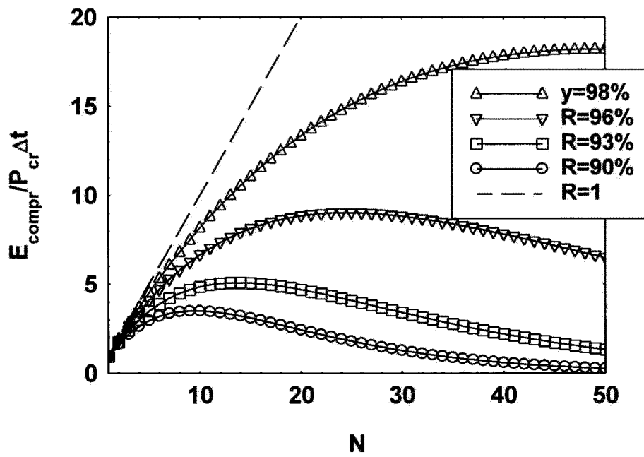
Compressed energy enchancement as a function of number of passes N
