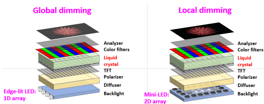
Global dimming and local dimming of thin-film transistor (TFT) liquid crystal displays
